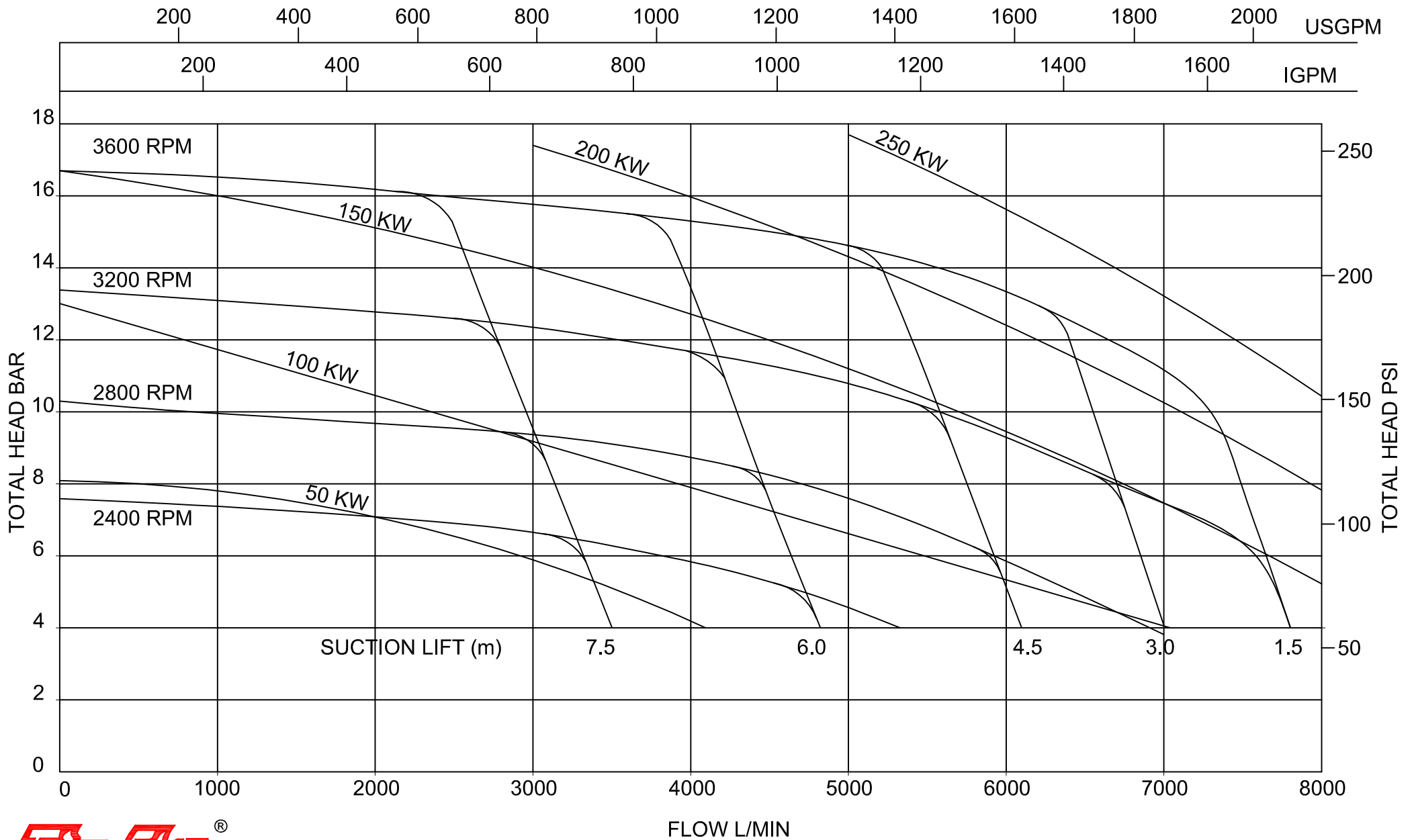
TYPICAL PERFORMANCE CURVE OF MFV MP 1060
